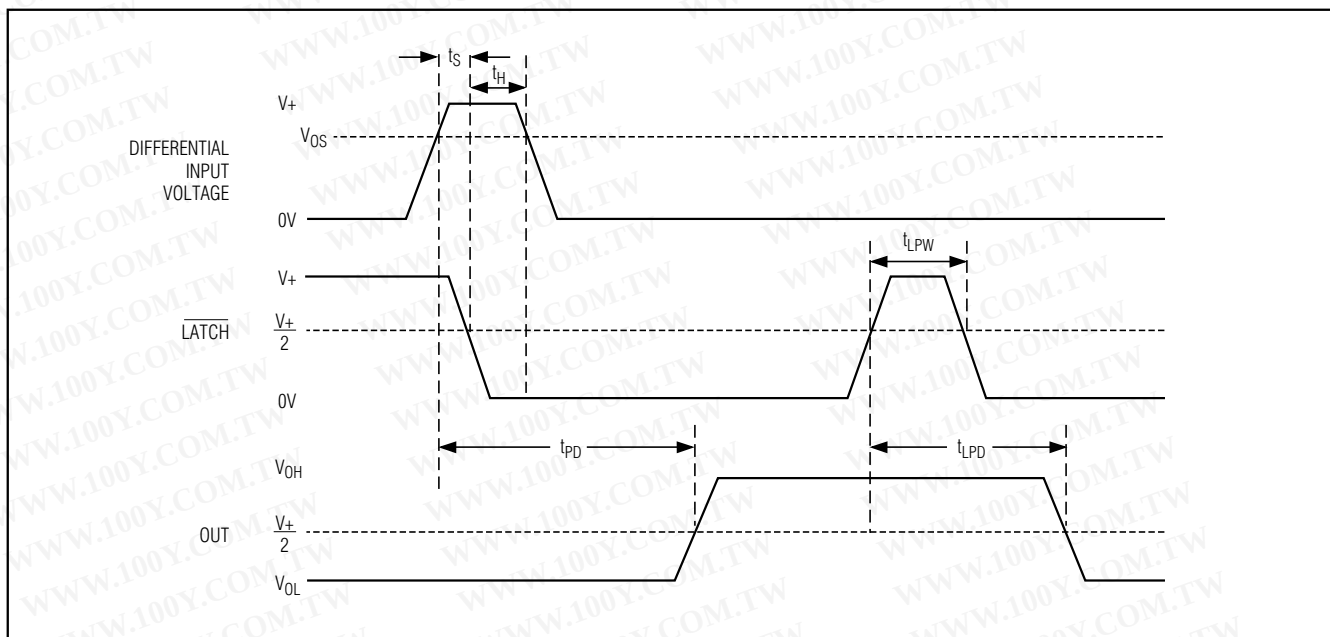
Figure 2. MAX941 Timing Diagram with Latch Operator
