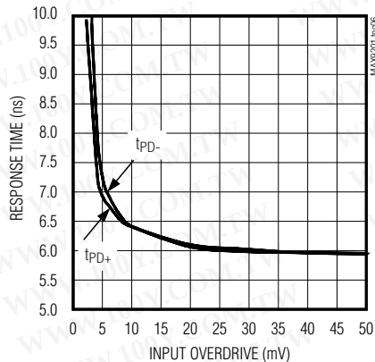
RESPONSE TIME vs. INPUT OVERDRIVE
