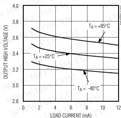
OUTPUT HIGH VOLTAGE ( V_{OH} ) vs. LOAD CURRENT
