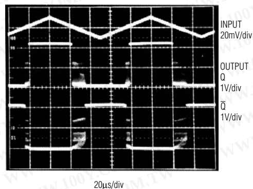
INDUSTRY-STANDARD 686 RESPONSE
