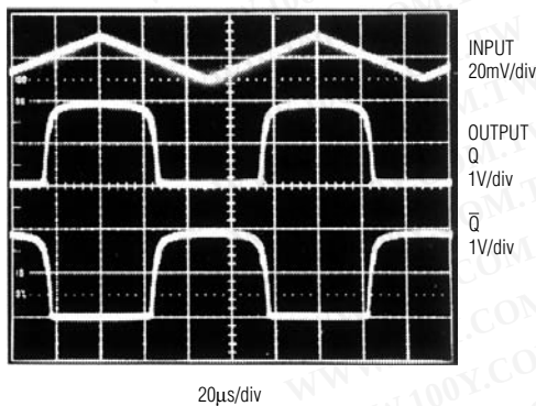
MAX912/MAX913 RESPONSE
