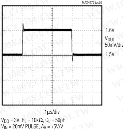
MAX4488/MAX4489 SMALL-SIGNAL PULSE RESPONSE
