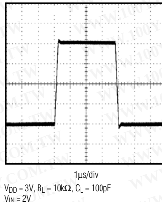
MAX4475-MAX4478 LARGE-SIGNAL PULSE RESPONSE
