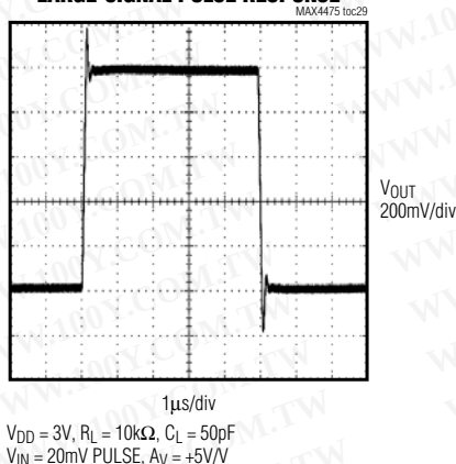
MAX4488/MAX4489 LARGE-SIGNAL PULSE RESPONSE
