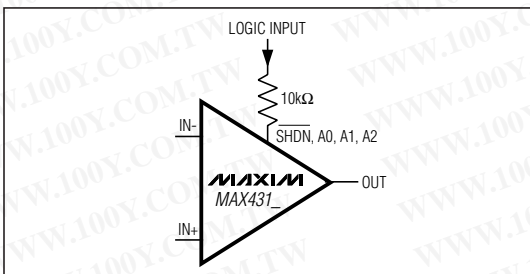
Figure 3. Circuit to Reduce Logic-Low Input Current
