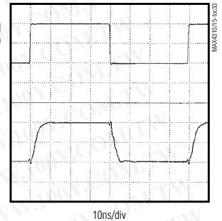
MAX4313 LARGE-SIGNAL PULSE RESPONSE
