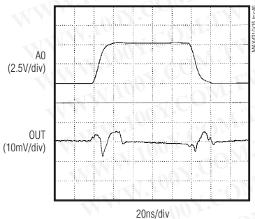
CHANNEL-SWITCHING TRANSIENT
