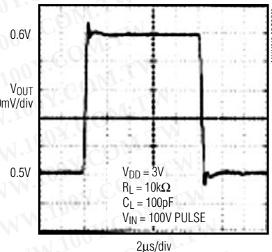
MAX4250-MAX4254 SMALL-SIGNAL PULSE RESPONSE
