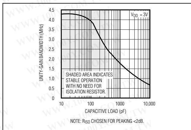
Figure 8. MAX4250–MAX4254 Unity-Gain Bandwidth vs. Capacitive Load
