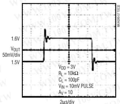
MAX4249/MAX4255/MAX4256/MAX4257 SMALL-SIGNAL PULSE RESPONSE
