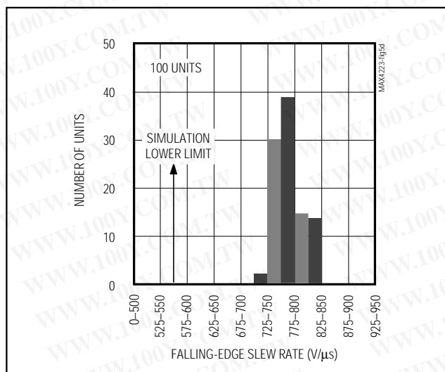
Figure 5d. MAX4223 Falling-Edge Slew-Rate Distribution
