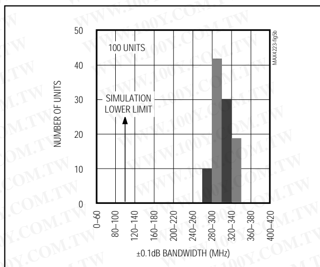
Figure 5b. MAX4223 ±0.1dB Bandwidth Distribution
