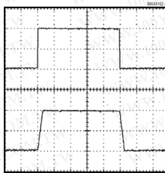
NONINVERTING LARGE-SIGNAL PULSE RESPONSE ( V_{DD} = 5V , C_L = 0 )
