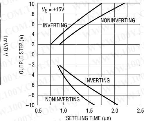
Settling Time to 0.01% vs Output Step
