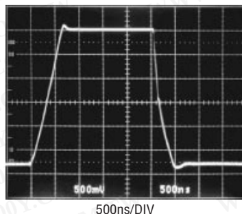
5V Large-Signal Response
