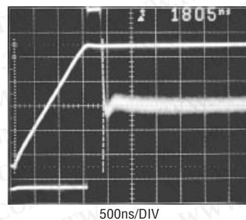
±15V Settling
