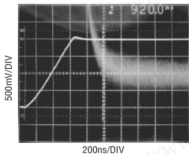
5V Settling
