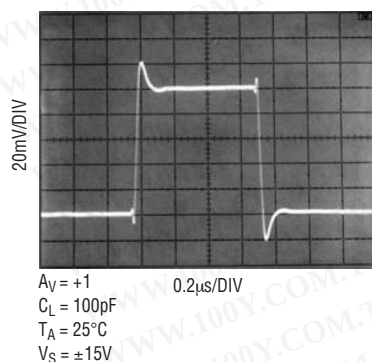
Small-Signal Response
