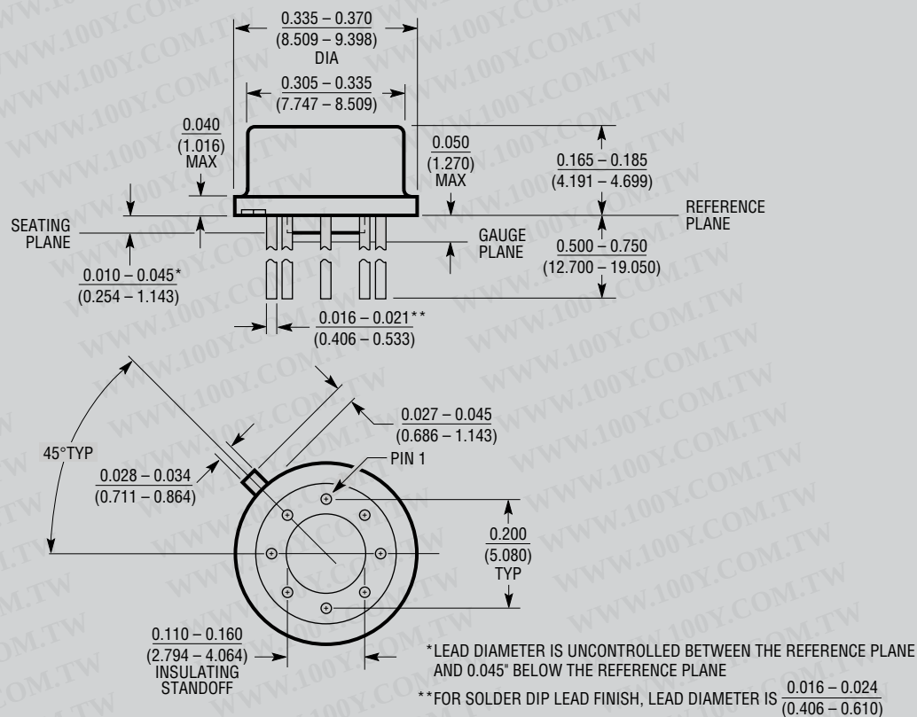
H Package 8-Lead TO-5 Metal Can (.200 Inch PCD) (Reference LTC DWG # 05-08-1320)
