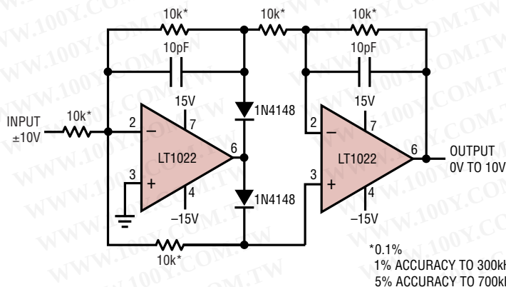
Wide Bandwidth Absolute Value Circuit
