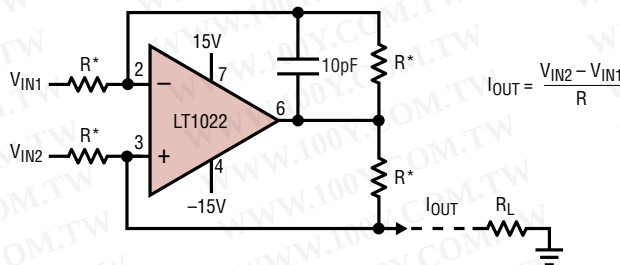
Fast, Differential Input Current Source
