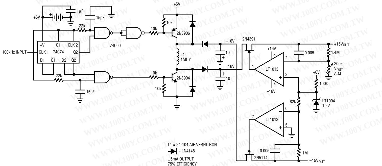
6V to \pm 15\text{V} Regulating Converter
