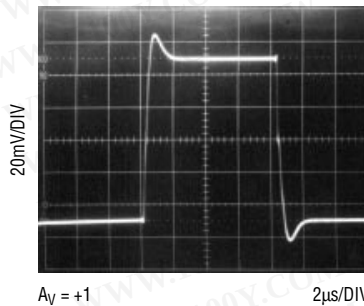
Small Signal Transient Response, VS = ±15V
