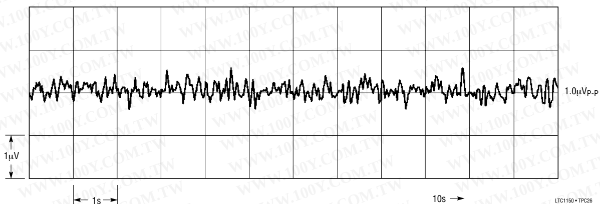
0.1Hz to 10Hz Noise, V = \pm 15V , T_A = 25^\circ C , f_S = 1800Hz
