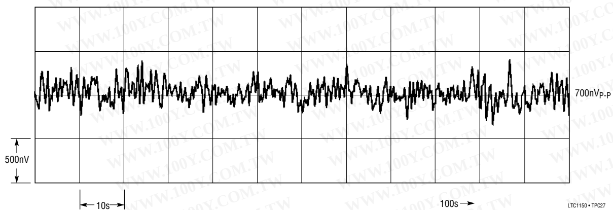
0.1Hz to 1Hz Noise, V = \pm 15V , T_A = 25^\circ C , Internal Clock
