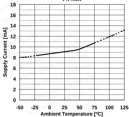
Supply Current vs. Temperature V^+/-V=\pm 15\text{V}
