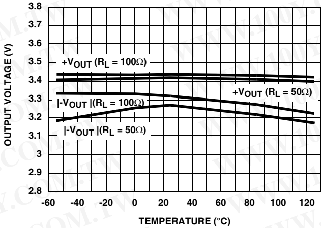
FIGURE 21. OUTPUT VOLTAGE vs TEMPERATURE
