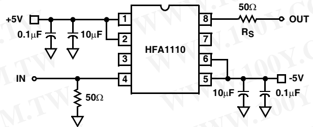
SCHEMATIC DIAGRAM
