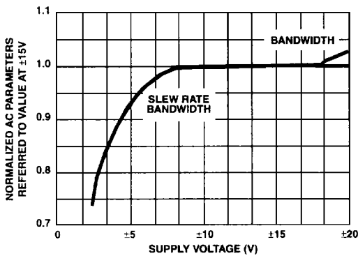
FIGURE 6. NORMALIZED AC PARAMETERS vs SUPPLY VOLTAGE
