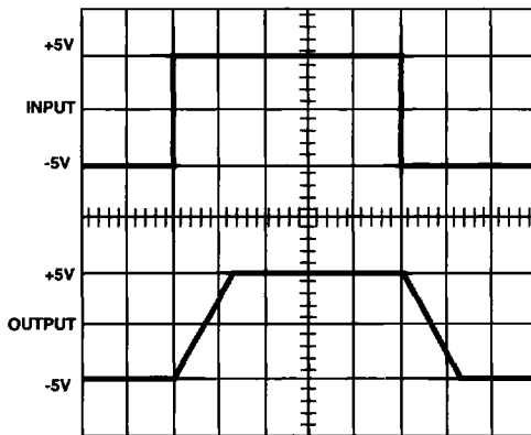
FIGURE 2. LARGE SIGNAL RESPONSE
