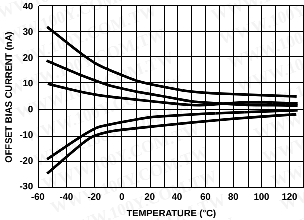
FIGURE 10. OFFSET BIAS CURRENT vs TEMPERATURE (5 TYPICAL UNITS FROM 3 LOTS)
