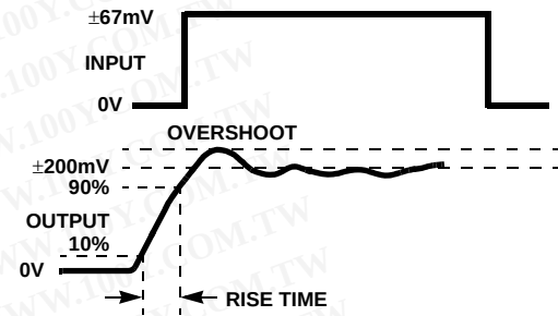
FIGURE 2. TRANSIENT RESPONSE
