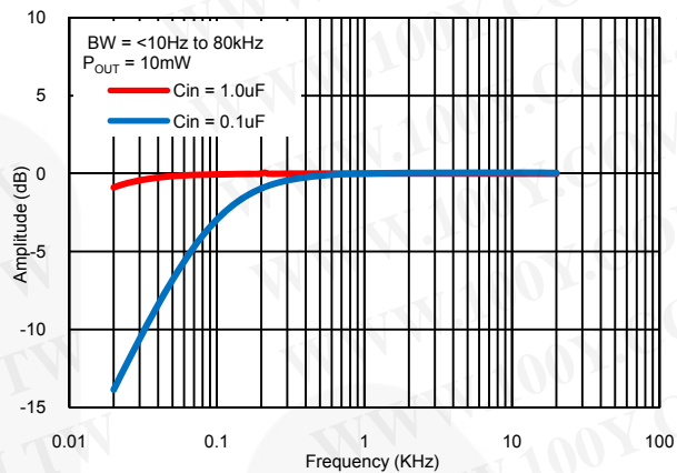
Figure 22. Frequency Response
