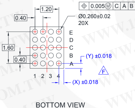
Figure 33. 20-Bump, Wafer-Level Chip-Scale Package (WLCSP), 0.4 mm Pitch
