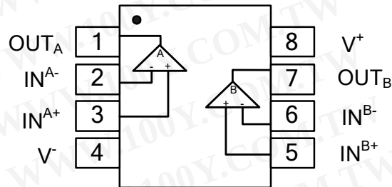
SOP-8L / MSOP-8L
