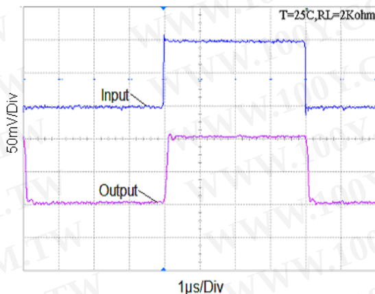
Non-Inverting Small Signal Pulse Response
