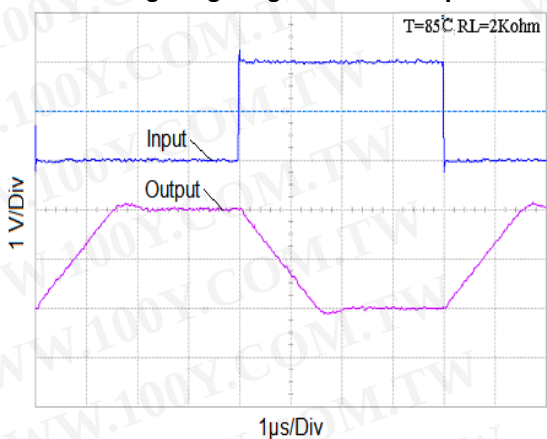
Inverting Large Signal Pulse Response
