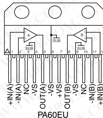
FIGURE 3. External connections
