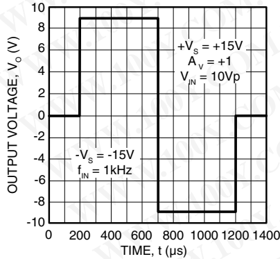
PULSE RESPONSE
