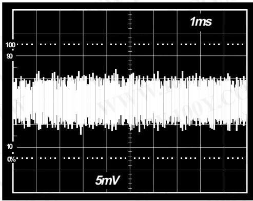
Figure 19. Voltage Noise from 0 kHz to 10 kHz*
