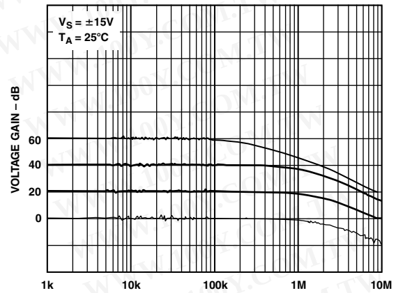
Figure 2. Bandwidth for Various Values of Gain
