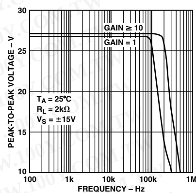
TPC 5. Maximum Output Swing vs. Frequency
