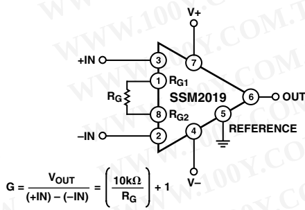
Figure 1. Basic Circuit Connections
