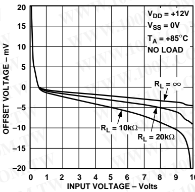
Figure 8. Offset Voltage vs. Input Voltage
