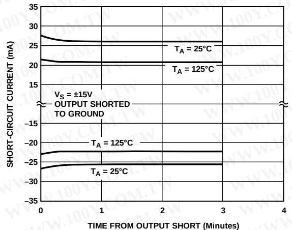
Figure 28. Short-Circuit Current vs. Time at Various Temperatures
