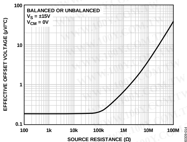
Figure 13. Effective TCV_{0S} vs. Source Resistance
