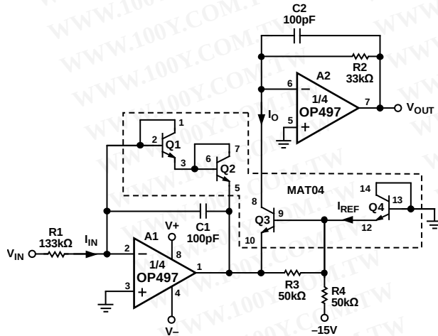
Figure 40. Squaring Amplifier
