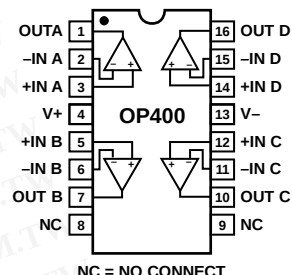
Figure 2. 16-Pin SOIC (S-Suffix)
