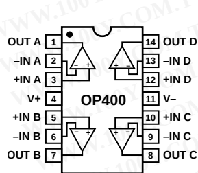
Figure 1. 14-Pin Ceramic DIP (Y-Suffix) and 14-Pin Plastic DIP (P-Suffix)
