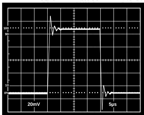
Figure 27. Small Signal Transient Response ( C_L = 1000 pF, A_{VCL} = +1 )
