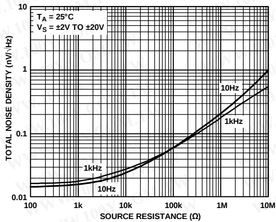
Figure 18. Total Noise Density vs. Source Resistance
