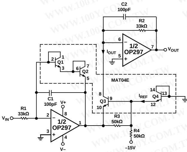
Figure 35. Squaring Amplifier
