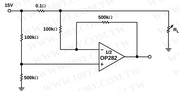
Figure 44. High-Side Signal Conditioning
