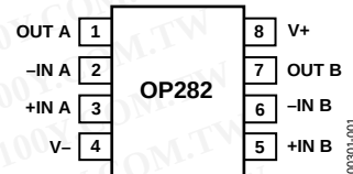
Figure 1. 8-Lead Narrow-Body SOIC (S-Suffix) [R-8]
