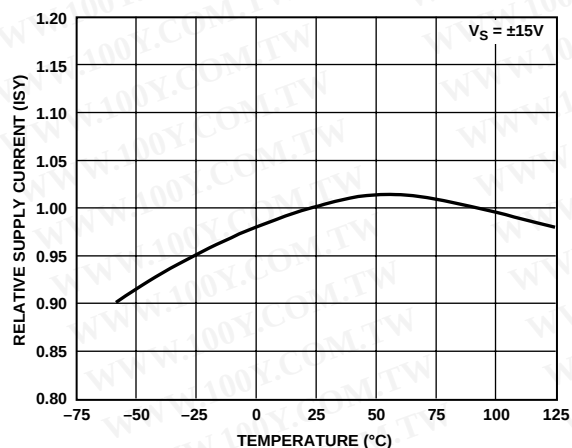
Figure 36. OP482 Relative Supply Current vs. Temperature
