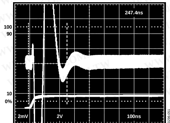
Figure 51. Transient Recovery Time of the OP249 from a 1 mA Load Transient to 0.01%
