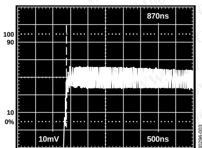
Figure 3. Fast Settling (0.01%)
