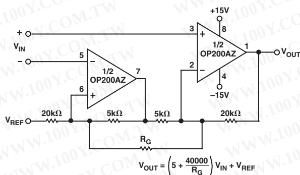
Figure 4. Dual Low Power Instrumentation Amplifier
