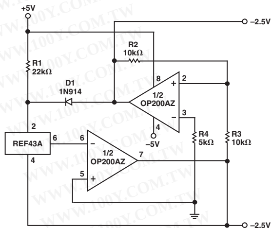
Figure 8. Dual Precision Voltage Reference
