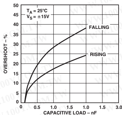
TPC 19. Overshoot vs. Capacitive Load
