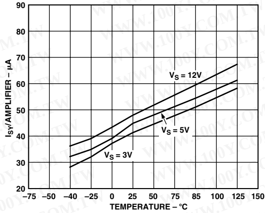
TPC 25. Supply Current/Amplifier vs. Temperature
