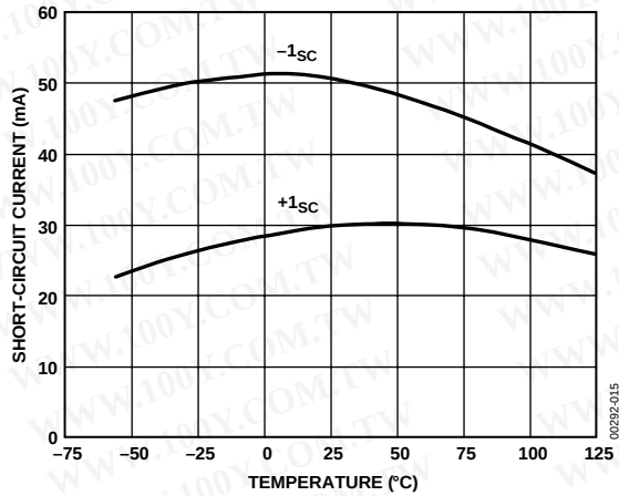
Figure 15. Short-Circuit Current vs. Temperature @ \pm 15 V
