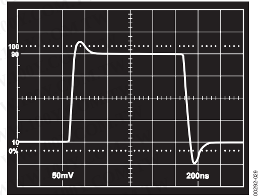
Figure 29. Small Signal Performance @ \pm 15 V
