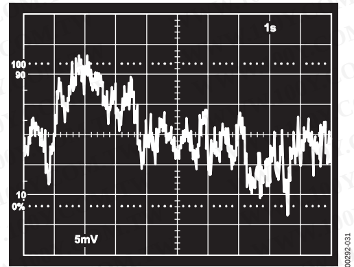
Figure 31. 0.1 Hz to 10 Hz Noise @ \pm 15 V
