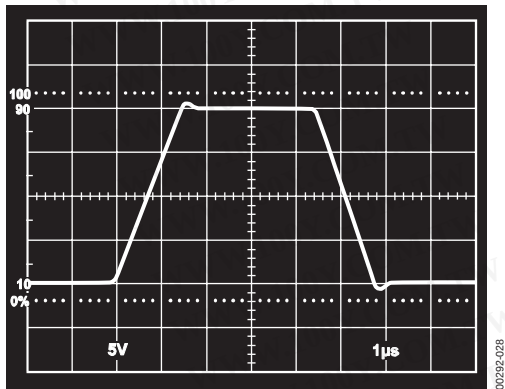
Figure 28. Large Signal Performance @ \pm 15 V
