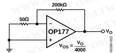
Figure 3. Typical Offset Voltage Test Circuit
