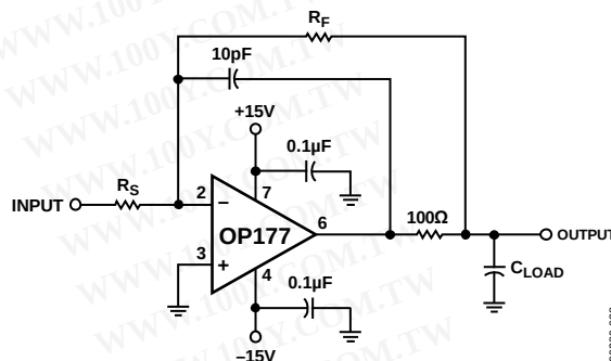
Figure 28. Isolating Capacitive Loads
