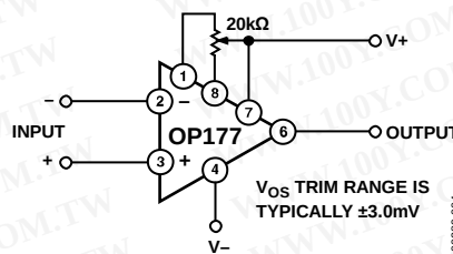
Figure 4. Optional Offset Nulling Circuit
