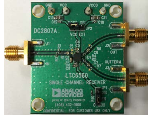
Figure 16. DC2807A Single Channel Electrical Evaluation Board
