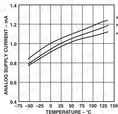
TPC 22. CMP402 Analog Supply Current vs. Temperature
