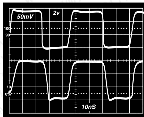
CMP401: 20 MHz Noninverting Switching, V_{IN} = \pm 100 mV
