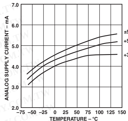
TPC 21. CMP401 Analog Supply Current vs. Temperature
