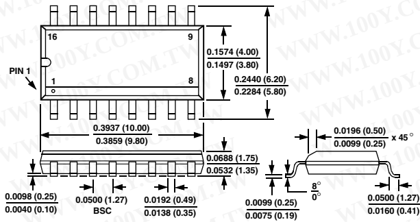
16-Lead Narrow-SOIC (R-16A)
