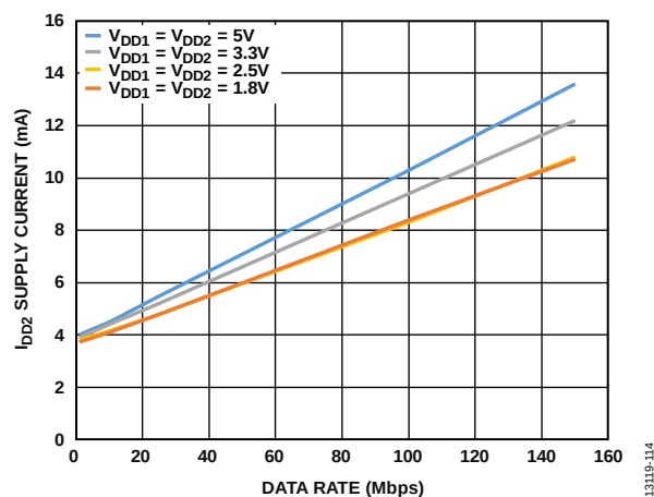
Figure 16. ADuM141D/ADuM141E I_{DD2} Supply Current vs. Data Rate at Various Voltages
