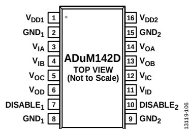
Figure 11. ADuM142D Pin Configuration
