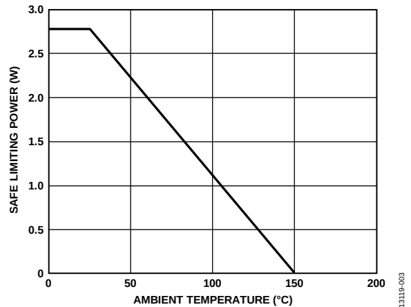
Figure 5. Thermal Derating Curve for RW-16 Wide Body [SOIC_W] Package, Dependence of Safety Limiting Values with Ambient Temperature per DIN V VDE V 0884-10
