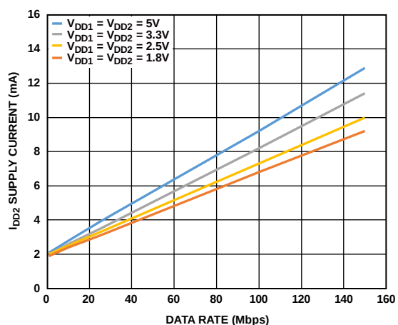
Figure 14. ADuM140D/ADuM140E I_{DD2} Supply Current vs. Data Rate at Various Voltages
