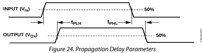
Figure 24. Propagation Delay Parameters
