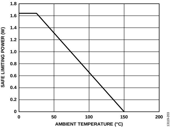
Figure 6. Thermal Derating Curve for RQ-16 [QSOP] Package, Dependence of Safety Limiting Values with Ambient Temperature per DIN V VDE V 0884-10
