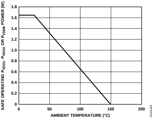
Figure 4. Thermal Derating Curve for R-16 Narrow Body [SOIC_N] Package, Dependence of Safety Limiting Values with Ambient Temperature per DIN V VDE V 0884-10
