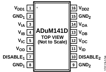
Figure 9. ADuM141D Pin Configuration
