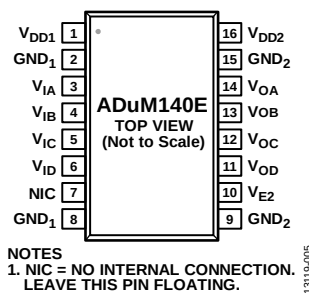
Figure 8. ADuM140E Pin Configuration
