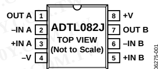
Figure 1. 8-Lead SOIC_N (R-8)
