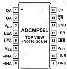
Figure 2. ADCMP561 16-Lead QSOP
