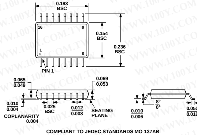
Figure 26. 16-Lead Shrink Small Outline Package [QSOP] (RQ-16) Dimensions shown in inches
