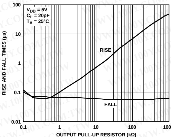
Figure 28. Rise and Fall Times vs. Output Pull-Up Resistor
