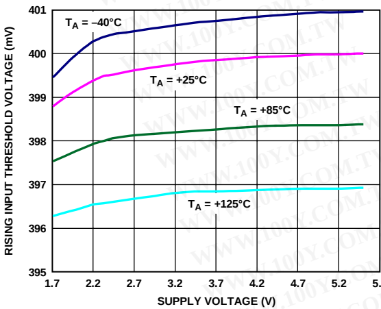
Figure 7. Rising Input Threshold Voltage vs. Supply Voltage
