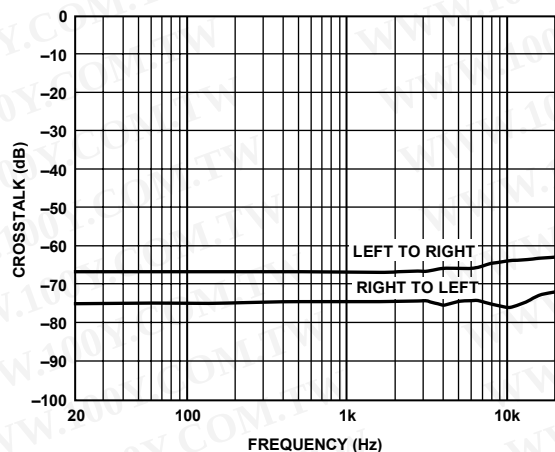
Figure 18. Crosstalk, 0 dBFS, 15 V, 8 \Omega
