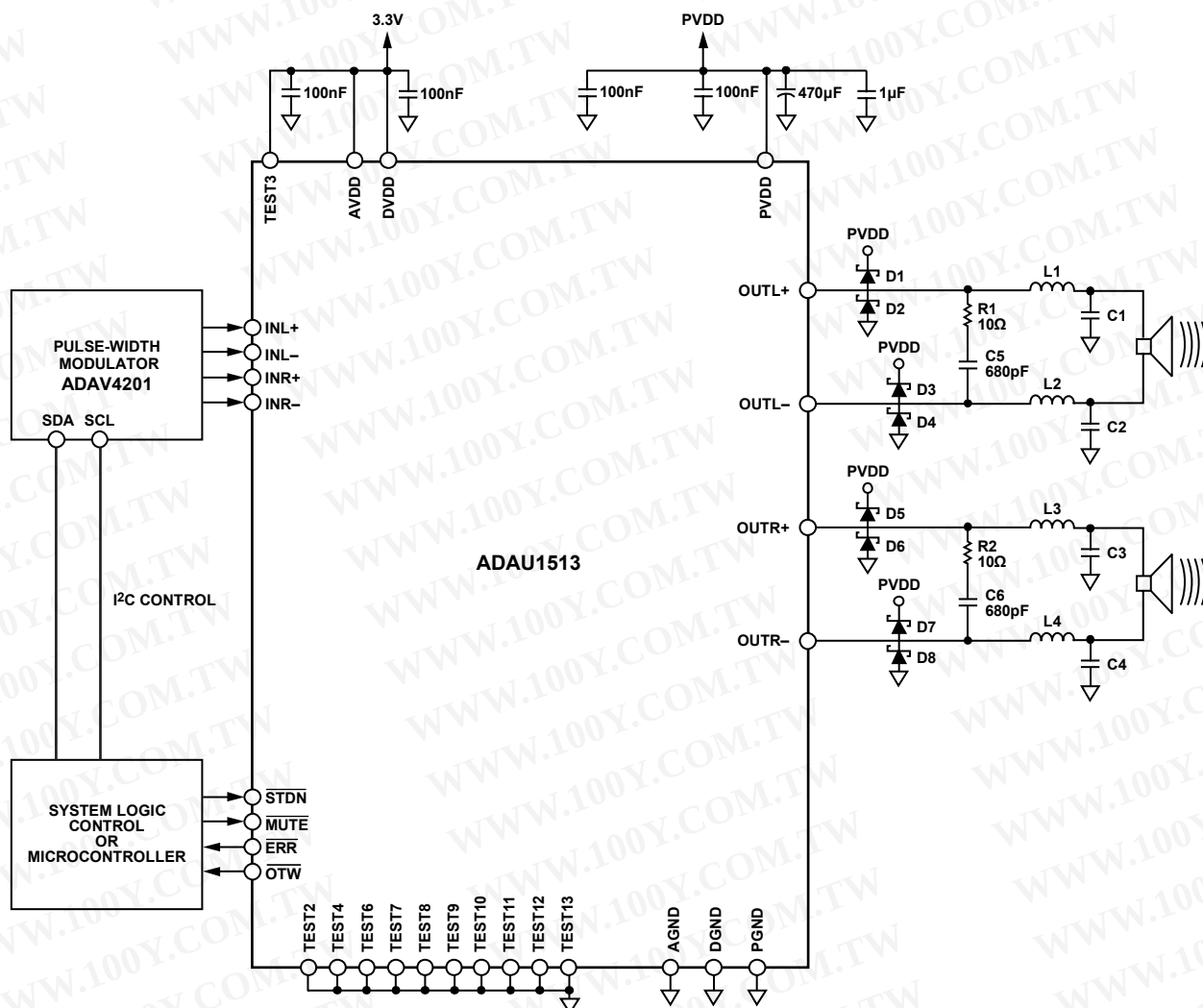
Figure 31. Application Schematic
