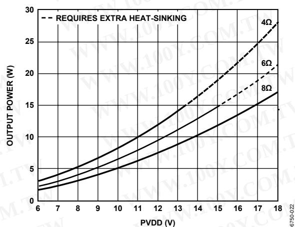
Figure 23. Output Power vs. PVDD, 40 dB THD + N
