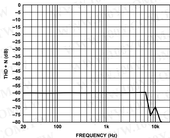
Figure 17. THD + N vs. Frequency, 1 W, 15 V, 8 \Omega
