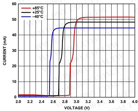
Figure 45. Supply Current vs. Power-Down Voltage and Temperature, V_S = 5\text{ V}
