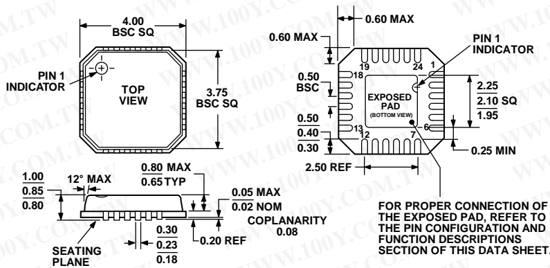
Figure 72. 24-Lead Lead Frame Chip Scale Package [LFCSQ_VQ] 4 mm × 4 mm Body, Very Thin Quad (CP-24-1) Dimensions shown in millimeters
