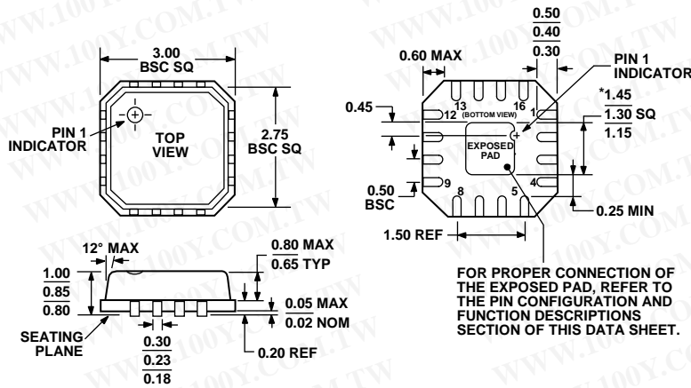
Figure 71. 16-Lead Lead Frame Chip Scale Package [LFCSQ_VQ] 3 mm × 3 mm Body (CP-16-2) Dimensions shown in millimeters
