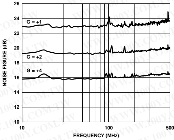
Figure 37. Noise Figure vs. Frequency
