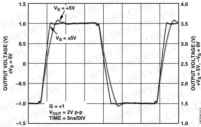
Figure 22. Large Signal Transient Response for Various Supplies
