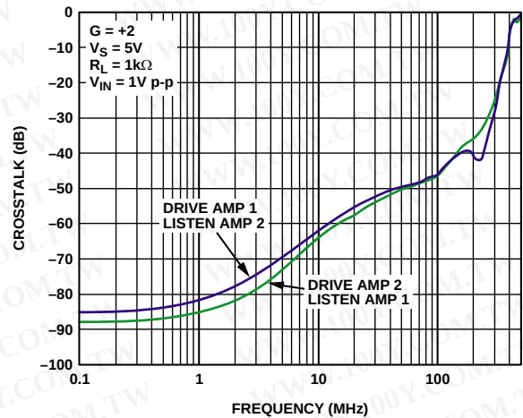
Figure 39. ADA4851-2, RTI Crosstalk vs. Frequency
