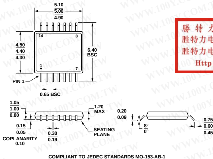
COMPLIANT TO JEDEC STANDARDS MO-153-AB-1 Figure 50. 14-Lead Thin Shrink Small Outline Package [TSSOP] (RU-14) Dimensions shown in millimeters
