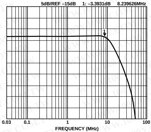
Figure 47. Video Reconstruction Filter Frequency Performance
