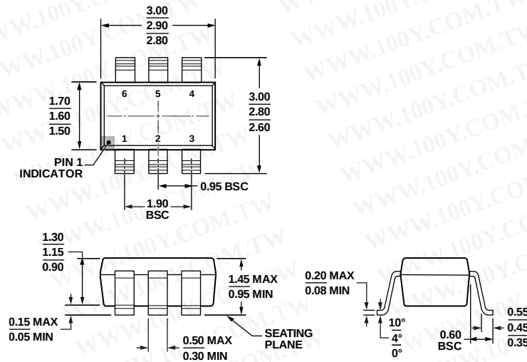
Figure 48. 6-Lead Small Outline Transistor Package [SOT-23] (RJ-6)
