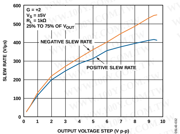
Figure 26. Slew Rate vs. Output Voltage Step
