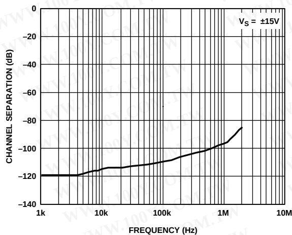
Figure 27. Channel Separation
