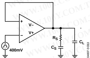
Figure 51. Snubber Network
