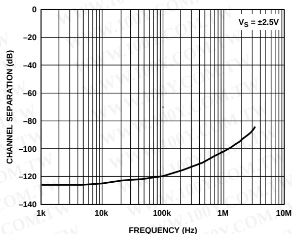
Figure 48. Channel Separation
