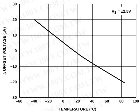
Figure 41. \Delta Offset Voltage vs. Temperature
