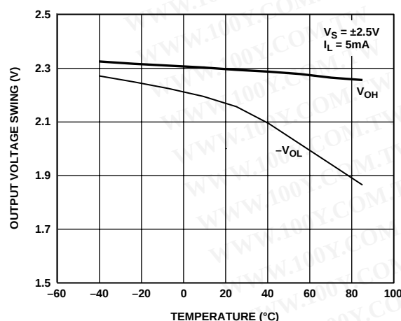
Figure 40. Output Voltage Swing vs. Temperature
