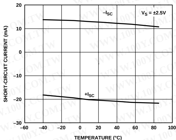
Figure 38. Short-Circuit Current vs. Temperature
