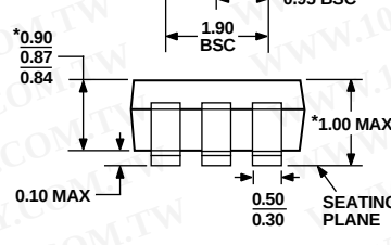
Figure 37. 5-Lead Thin Small Outline Transistor Package [TSOT] (UJ-5)
