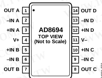
Figure 6. 14-Lead TSSOP
