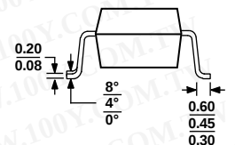
Figure 37. 5-Lead Thin Small Outline Transistor Package [TSOT] (UJ-5)
