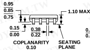
Figure 34. 8-Lead Mini Small Outline Package [MSOP] (RM-8)
