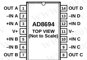
Figure 5. 14-Lead SOIC
