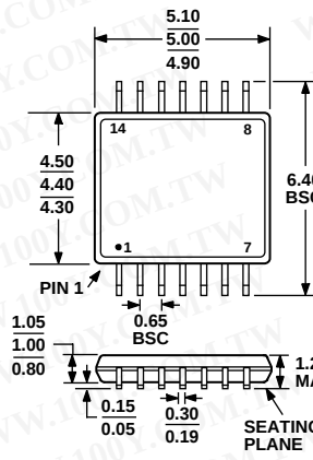
Figure 38. 14-Lead Thin Shrink Small Outline Package [TSSOP] (RU-14)
