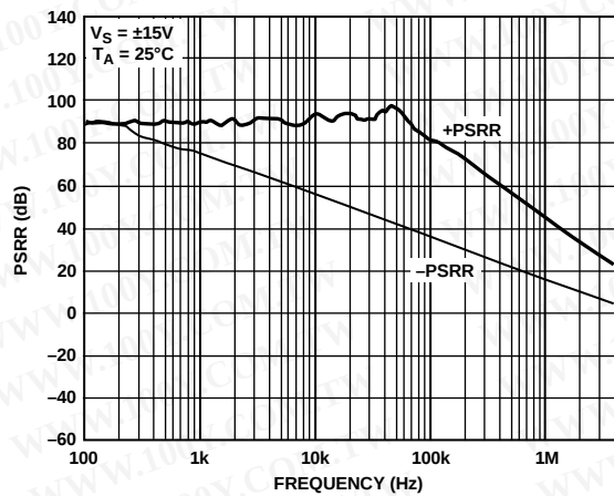
Figure 16. AD8682 PSRR vs. Frequency
