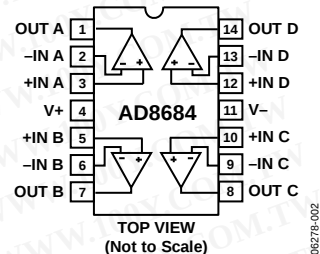
Figure 2. 14-Lead SOIC_N and 14-Lead TSSOP
