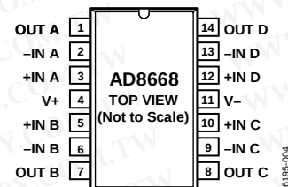
Figure 6. AD8668, 14-Lead SOIC_N (R-14)
