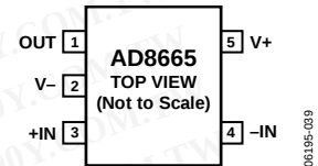
Figure 1. AD8665, 5-Lead SOT-23 (RJ-5)
