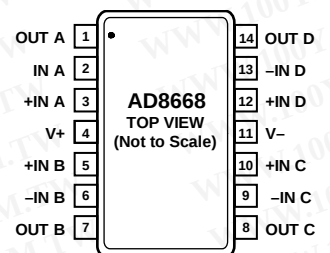
Figure 5. AD8668, 14-Lead TSSOP (RU-14)
