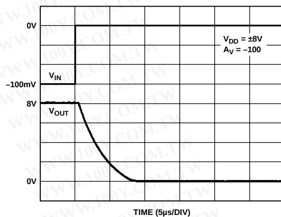
Figure 22. Positive Overload Recovery Time
