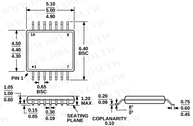
Figure 43. 14-Lead Thin Shrink Small Outline Package [TSSOP] (RU-14) Dimensions shown in millimeters
