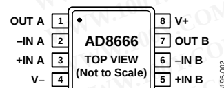
Figure 4. AD8666, 8-Lead MSOP (RM-8)
