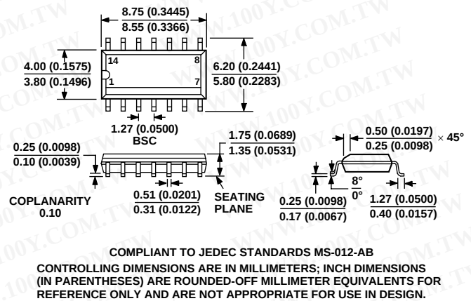
Figure 44. 14-Lead Standard Small Outline Package [SOIC_N] Narrow Body (R-14) Dimensions shown in millimeters and (inches)
