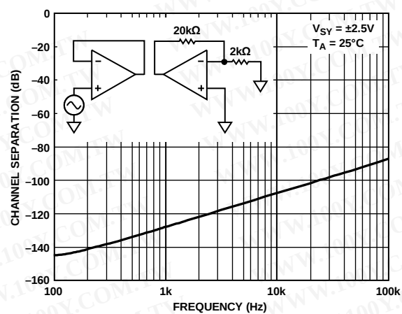
Figure 41. Channel Separation vs. Frequency
