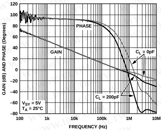
Figure 18. Open-Loop Gain and Phase Shift vs. Frequency
