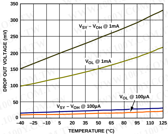
Figure 17. Output Voltage Saturation vs. Temperature
