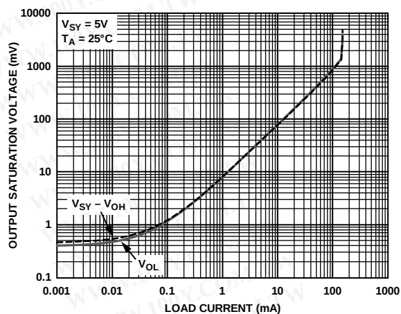
Figure 13. Output Saturation Voltage vs. Load Current
