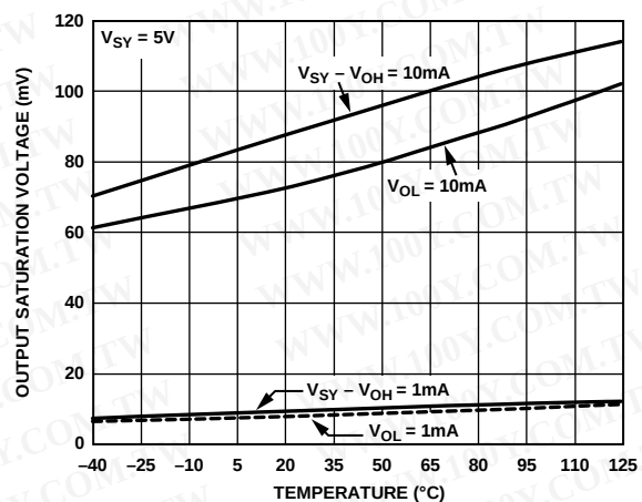
Figure 14. Output Saturation Voltage vs. Temperature
