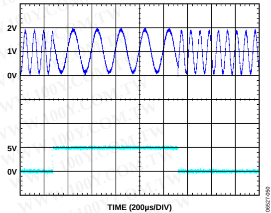
Figure 49. Switching Waveforms
