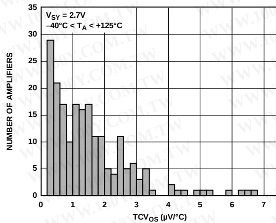
Figure 5. V_{OS} Drift ( TCV_{OS} ) Distribution
