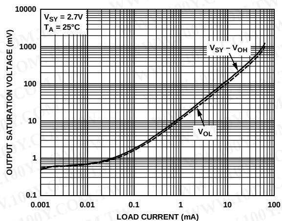
Figure 10. Output Saturation Voltage vs. Load Current
