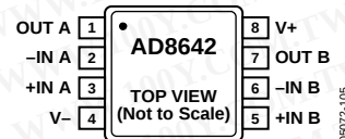
Figure 3. 8-Lead SOIC (R-8)
