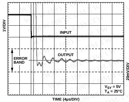
Figure 35. Negative Settling Time to 0.1% 5V
