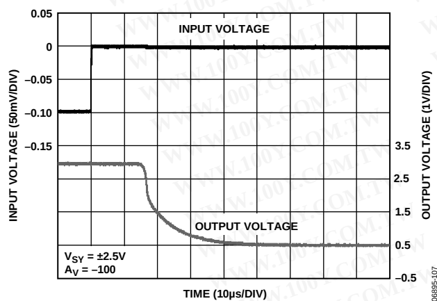
Figure 29. Negative Overload Recovery
