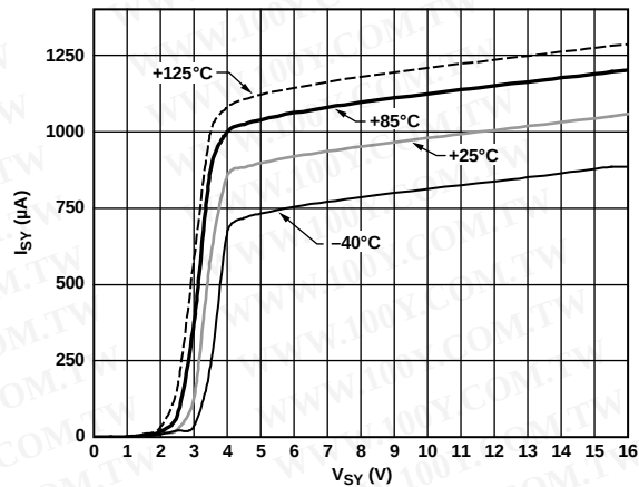
Figure 42. Supply Current vs. Supply Voltage
