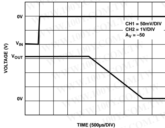
Figure 61. Negative Input Overload Recovery for Competitor B
