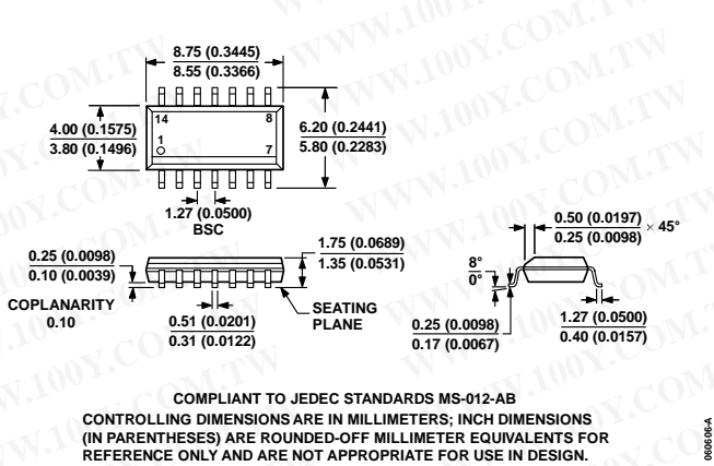
Figure 69. 14-Lead Standard Small Outline Package [SOIC_N] Narrow Body (R-14) Dimensions shown in millimeters and (inches)
